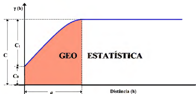
Figura 2- Semivariograma experimental.
